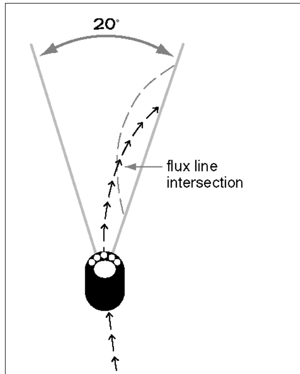
Figure 8. Avoiding "Jumped Flux Lines." Sometimes flux lines can intersect within the Tracker's 20-degree Special mode window. As you move through the intersection, pay attention to your distance and direction displays—especially the LED's just the the left and right of center. Do not deviate from the established curve of your intended flux-line search .
