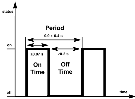
Figure 4. Pulse Rates. The ETS 300 718 standards on pulse periods and pulse widths are shown above. For an illustration of how widely these standards can vary, see Figure 5, below.
