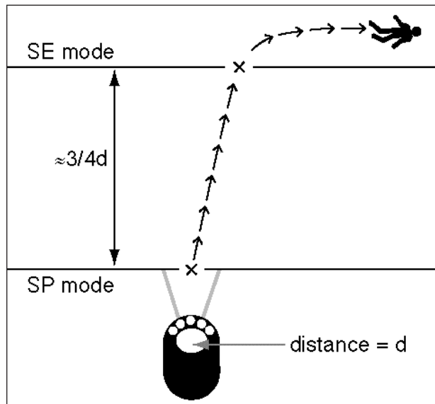
Figure 10. Isolating/locking in signals. To "break away" from the first transmitter, isolate the next signal in Special (SP) mode. Travel approximately 3/4 the distance shown. It is helpful to travel just far enough in Special mode to confirm the distance is decreasing and toward which direction the flux line is trending. Once this approximate distance is covered, re-enter Search (SE) mode to lock in the next transmitter.
